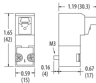
90° Connector with LED
