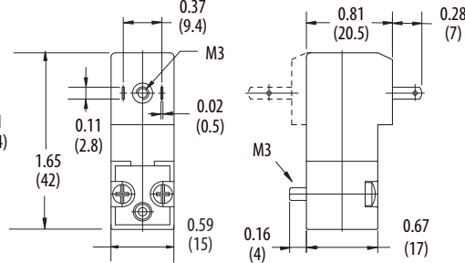
Terminal Connector (Ind. Form)
